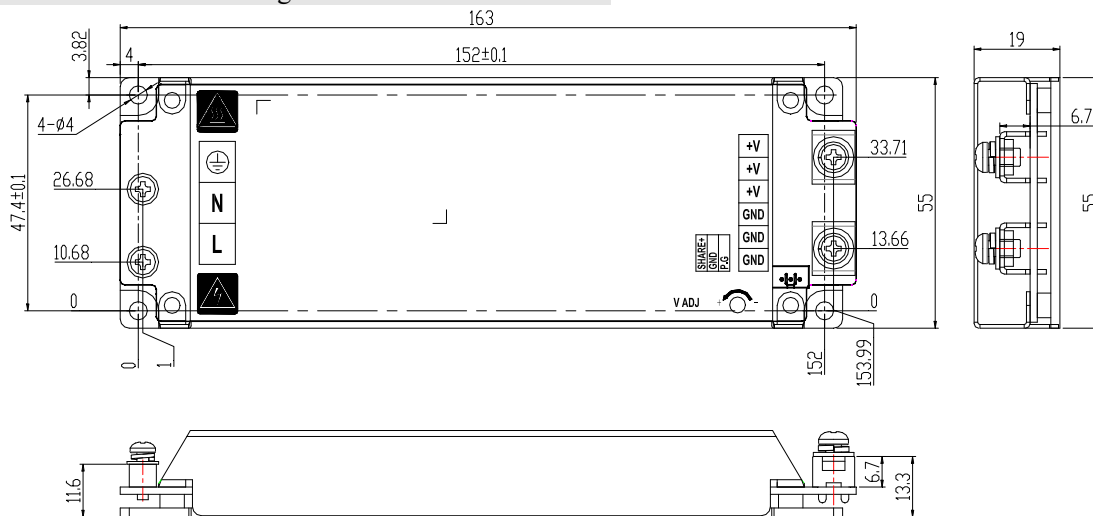
Dimensions and mounting holes - terminal coordinates
